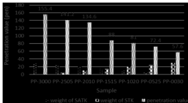
Figure 1. Penetration test of the hat-adsorbing materials
