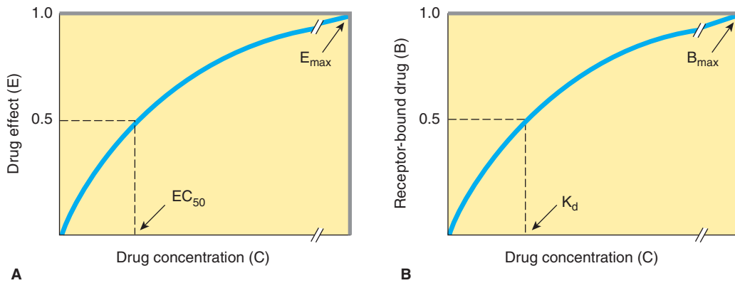
FIGURE 2-1 Relations between drug concentration and drug effect (A) or receptor-bound drug (B). The drug concentrations at which effect or receptor occupancy is half-maximal are denoted by EC 50 and K d , respectively.
