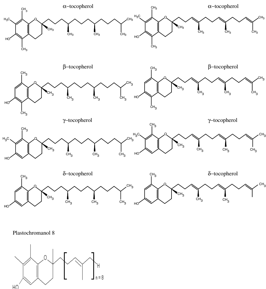
Figure 11.1 Structures of common tococls.
