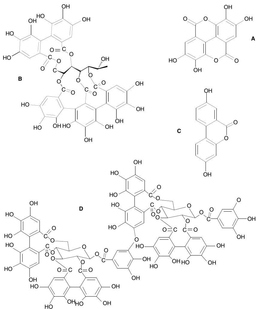
Figure 6.1 Common structures associated with ellagitannins include (A) free ellagic acid (hydrolytic product), (B) castalagin (oak wood), (C) Urolithin A (fecal metabolite), and (D) dimeric Sanguiniin H-6 ( Rubus species).
