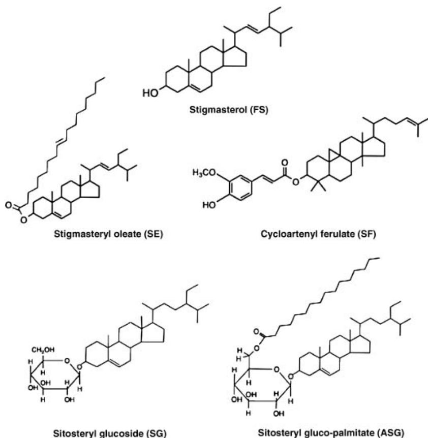
Figure 10.1 Examples of structural formulas of phytosterol and sterol conjugates. FS = free sterol alcohol, SE = sterol fatty acid ester, SF = steryl ferulate, SG = steryl glycoside, ASG = acylated steryl glycoside.
