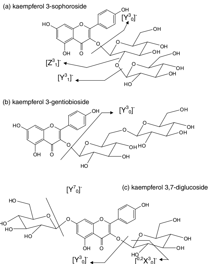
Figure 7.8B MS2[M-H] - fragmentation patterns of isomeric flavonol diglucosides (Ferrerres et al., 2004).
