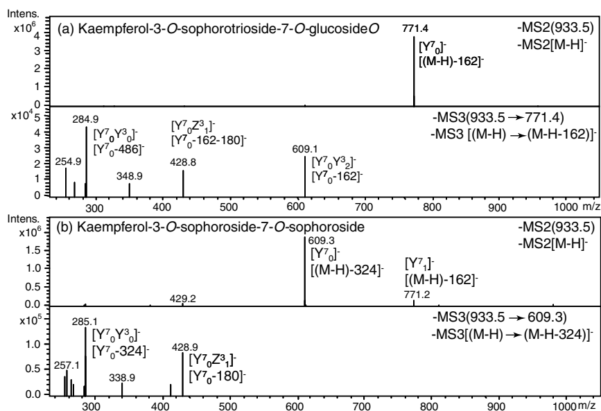
Figure 7.7 \text{MS}_2[\text{M}-\text{H}]^- and \text{MS}_3[(\text{M}-\text{H}) \rightarrow \text{Y}_0^7]^- of isomeric flavonol tetraglucosides: (a) kaempferol-3-O-sophorotrioside-7-O-glucoside; (b) kaempferol-3-O-sophoroside-7-O-sophoroside (Ferrerres et al., 2004).
