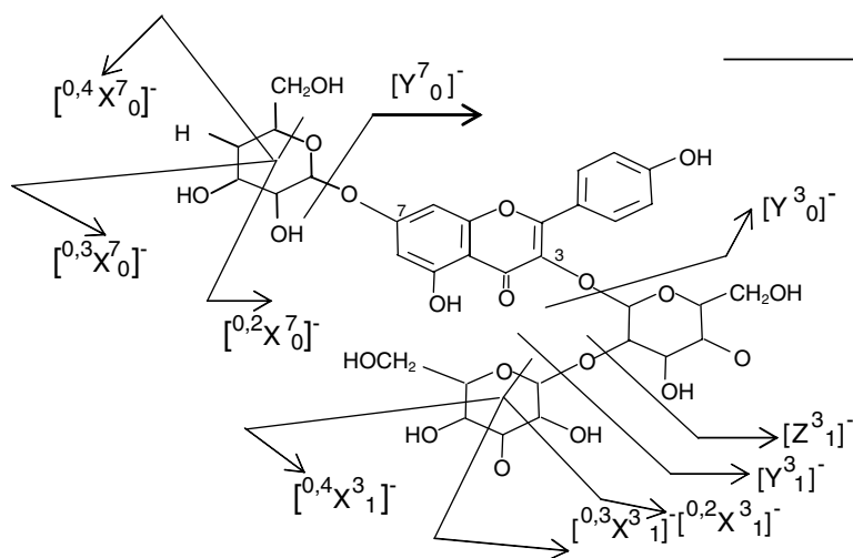
Figure 7.6 General scheme of the MS fragmentations of flavonoid glycosides.
