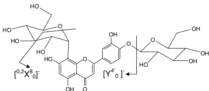
Figure 7.12 MS2[M-H] - and MS3[(M-H) \rightarrow Y 0 ] - of C-glycosyl flavones O-glycosylated on phenolic hydroxyl: (a) 4'-O-glucosyl-6-C-glucosyl luteolin; (b) 4'-O-glucosyl-8-C-glucosyl luteolin (Ferrerres et al., 2007b).
