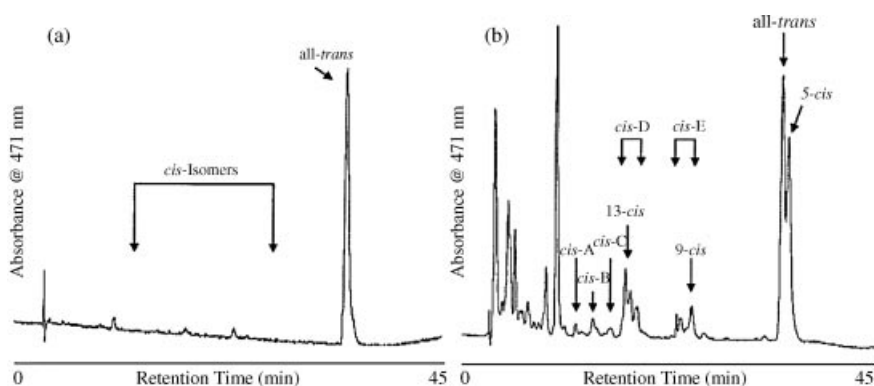
Figure 4.5 Representative HPLC chromatogram of (a) tomato product lycopene isomers in (b) plasma lycopene isomers from healthy individuals consuming different lycopene-containing tomato products for 15 days, demonstrating the presence of isomers in human blood plasma versus the all- trans form found in most foods (Hadley et al., 2003).
