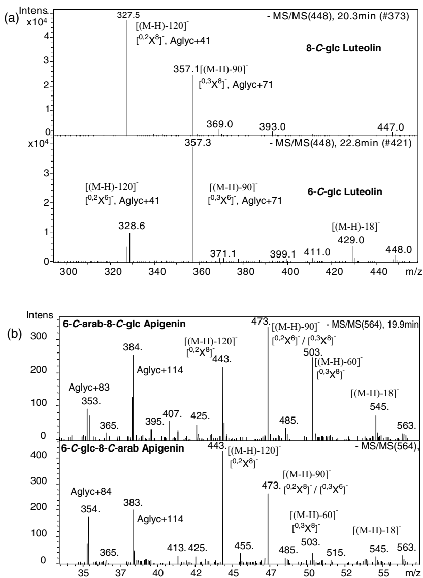
Figure 7.10 MS 2 [M-H] - of (a) mono-C-glycosyl flavonoid isomers: 8-C-glucosyl luteolin and 6-C-glucosyl luteolin and (b) asymmetric di-C-glycosyl flavone isomers: 6-C-arabinosyl-8-C-glucosyl apigenin and 6-C-glucosyl-8-C-arabinosyl apigenin (Ferrerres et al., 2003).
