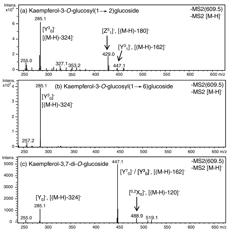
Figure 7.8A HPLC ESI-MS-MS analysis (MS2[M-H] - ) of isomeric flavonol diglucosides: (a) kaempferol-3- O -sophoroside (glucosyl(1-2)glucoside); (b) kaempferol-3- O -gentiobioside (glucosyl(1-6)glucoside); (c) kaempferol-3,7-di- O -glucoside (Ferrerres et al., 2004).
